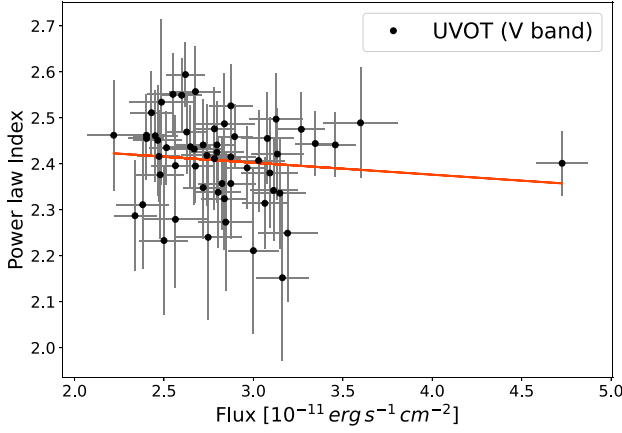
Figure 4. Left: Correlation between the optical flux in the V band and the photon index in the optical-to-UV band measured by UVOT. Right: Correlation between the X-ray flux in the 0.3–10, and 2–10 keV energy bands and the photon indexes measured with Swift-XRT and that in the 3–78 keV band as measured with NuSTAR. A clear break emerges between the two energetic regimes. In both panels, the dashed lines show the average trend of the data and were obtained with a linear fit.
