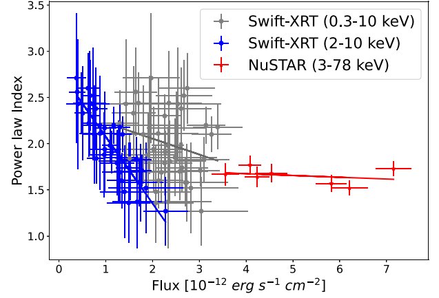
Figure 4. Left: Correlation between the optical flux in the V band and the photon index in the optical-to-UV band measured by UVOT. Right: Correlation between the X-ray flux in the 0.3–10, and 2–10 keV energy bands and the photon indexes measured with Swift-XRT and that in the 3–78 keV band as measured with NuSTAR. A clear break emerges between the two energetic regimes. In both panels, the dashed lines show the average trend of the data and were obtained with a linear fit.
