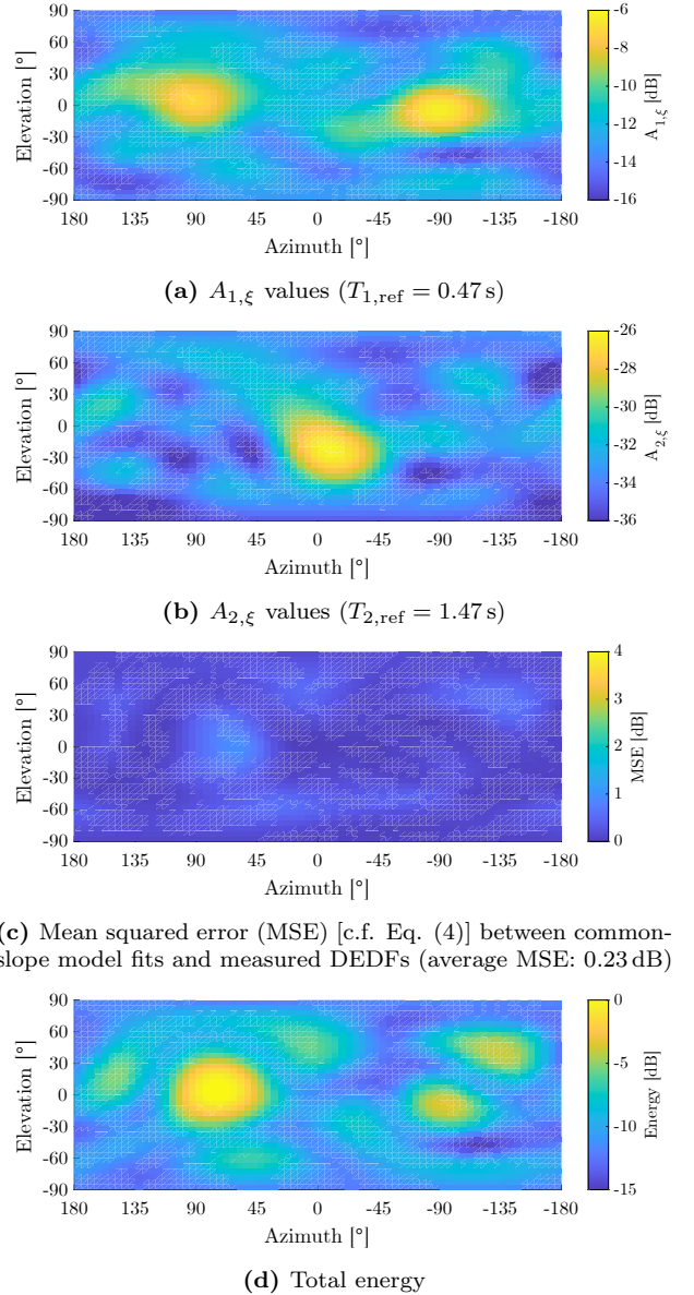
Figure 4: Common-slope amplitude and total energy variation across different directions for a coupled room measurement. The analysis is based on the DEDFs in the 1 kHz octave band and uses a maximum spherical harmonics order N_{\text{sph}} = 4 and decay model order K = 2 .
