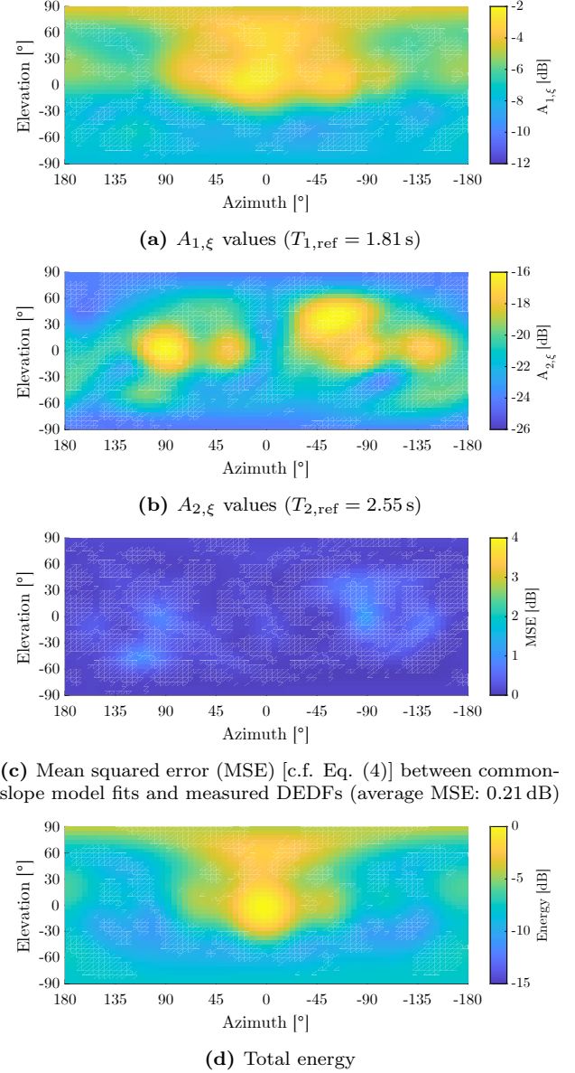
Figure 2: Common-slope amplitude and total energy variation across different directions for a concert hall measurement. The analysis is based on the DEDFs in the 1 kHz octave band and uses a maximum spherical harmonics order N_{sph} = 4 and decay model order K = 2 .
