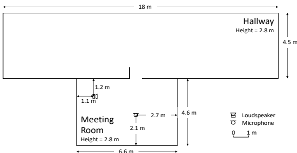
Figure 3: Coupled room measurement setup [9].
