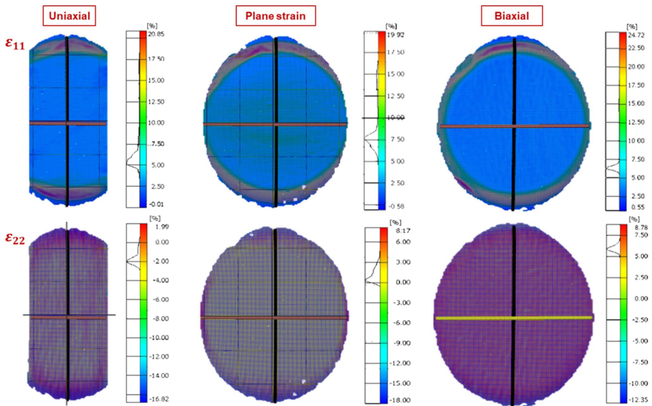
Fig. 5 The distribution of the major strain ( \epsilon_{11} ) and minor strain ( \epsilon_{22} ) of the center of Marciniak samples after uniaxial, plane-strain, and biaxial tension pre-loading measured by DIC
