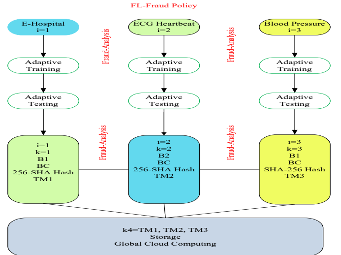
Fig. 2: Federated Learning Fraud-Detection Analysis and Policy.
