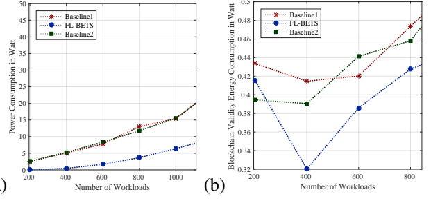
Fig. 5: Energy Consumption of IoMT During Fraud Analysis and Execution With Different Numbers of Tasks.
