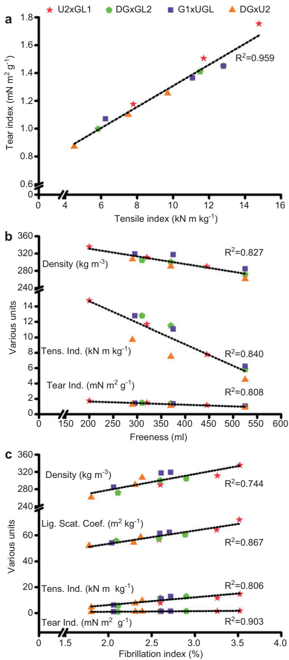
Figure 2 Summary of physical, mechanical, optical, and morphologic properties for all three refining levels from the four Eucalyptus hybrid pulp samples investigated.
