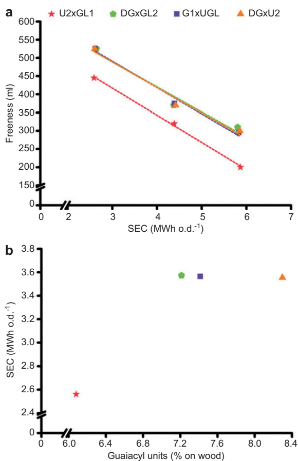
Figure 1 Relation of the SEC to (a) freeness (Canadian Standard Freeness) and (b) guaiacyl units at the freeness level of 450 ml in Eucalyptus hybrids.
