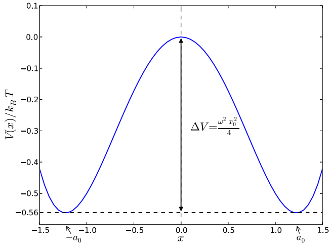
FIG. 1. The external potential of Eq. (4). The maximum of height \Delta V = \omega^2 a_0^2/4 \approx 0.56 is located at x=0 and the symmetric minima are located at x = \pm a_0 \approx \pm 1.22 . The initial state, I, is confined to the left well x < 0 and the right well x > 0 corresponds to the final state, F.
