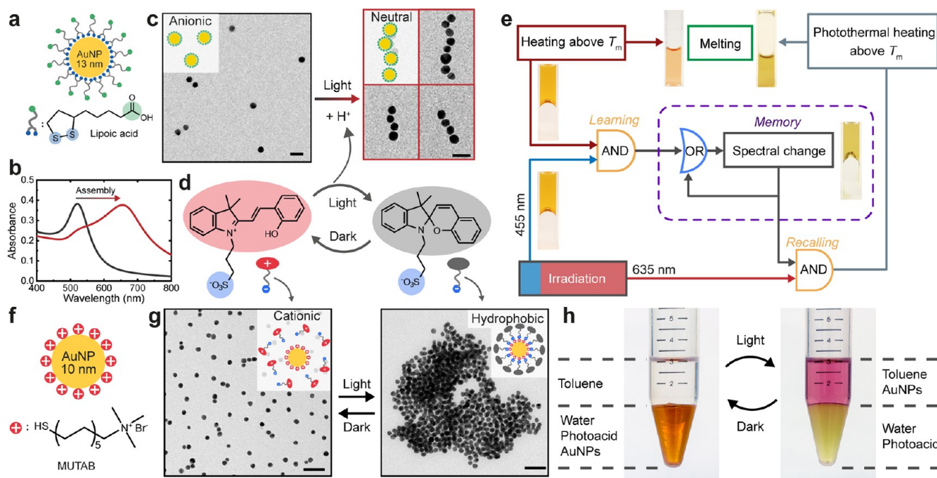
Figure 5. (a) AuNPs modified with lipoic acid (LA-AuNPs). (b) UV–vis spectra of dispersed (black) and assembled (red) LA-AuNPs. (c) TEM images showing the linear self-assembly of LA-AuNPs induced by light-triggered pH change. Scale bars 30 nm. (d) Illustration of the light induced isomerization of the photoacid. Upon irradiation, a proton is released, accompanied by the zwitterionic–anionic transition of the photoacid molecule. (e) Logic diagram of the response in an agarose network containing LA-AuNPs and photoacid, which shows classical conditioning behavior in response to light and heat. (f) Cationic AuNPs modified with (11-mercaptopundecyl)- N,N,N -trimethylammonium bromide (MUTAB). (g) TEM images showing the light-induced reversible hydrophobization of the cationic AuNPs due to adsorption/desorption of the photoacid. Scale bars 50 nm. (h) Photographs showing reversible transfer of cationic AuNPs between water and toluene. Panels a–c and e reproduced with permission from ref 4. Published 2019 by Springer Nature Ltd. Panels d and f–h reproduced with permission from ref 90. Copyright 2019 Royal Society of Chemistry.
