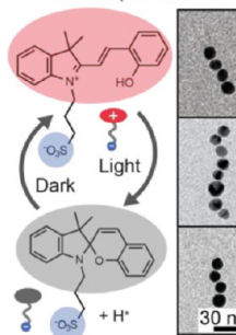
Light-controlled assembly of nanoparticles
