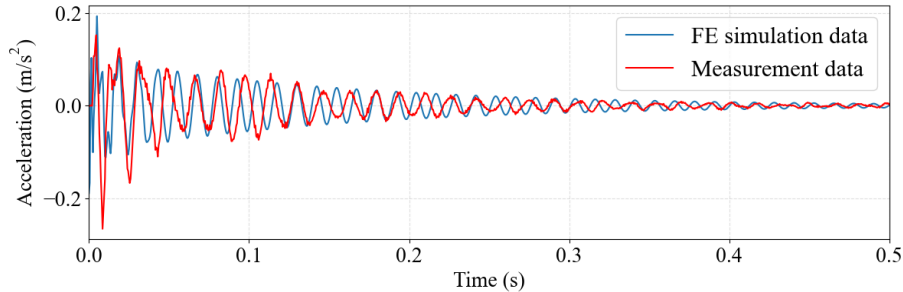
Fig. 7. Comparison between the FE simulation data and measurement data
