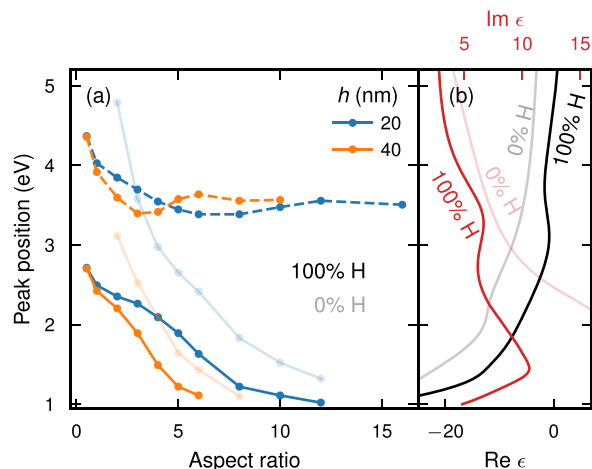
Figure 3. Peak position of the two peaks in the extinction spectra for PdH (opaque lines) and Pd (transparent lines) as a function of aspect ratio for two disk heights h (a) and the corresponding dielectric functions (b). PdH displays two features, one low-energy peak (solid line) which shifts with aspect ratio and one high-energy peak (dashed lines) which only shifts for small aspect ratios, indicating avoided-crossing behavior due to coupling between the peaks. The high-energy peak can be traced to the feature at 3.5 eV in the dielectric function (b) for 100% H (opaque line). This feature is not present for 0% H (transparent line), and as a result, the LSPR peak can shift over a much wider energy interval (transparent lines in b). Note that (b) shows the fitted Lorentzian representation of the dielectric functions.
