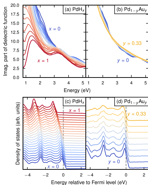
Figure 1. Variation of the imaginary part of the dielectric function as a function of photon energy for (a) \text{PdH}_x without Au and (b) \text{Pd}_{1-y}\text{Au}_y in the absence of H, as calculated in this work. The dielectric function is closely related to the density of states (c, d). Energies have been shifted such that the Fermi level is always at 0 eV.
