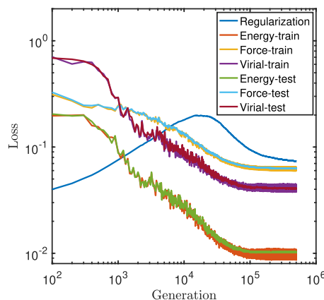
FIG. 2. Evolution of the various terms in the loss function (33) with respect to the generation in the SNES 58 training algorithm for the MgAlCu training and test datasets. 123
