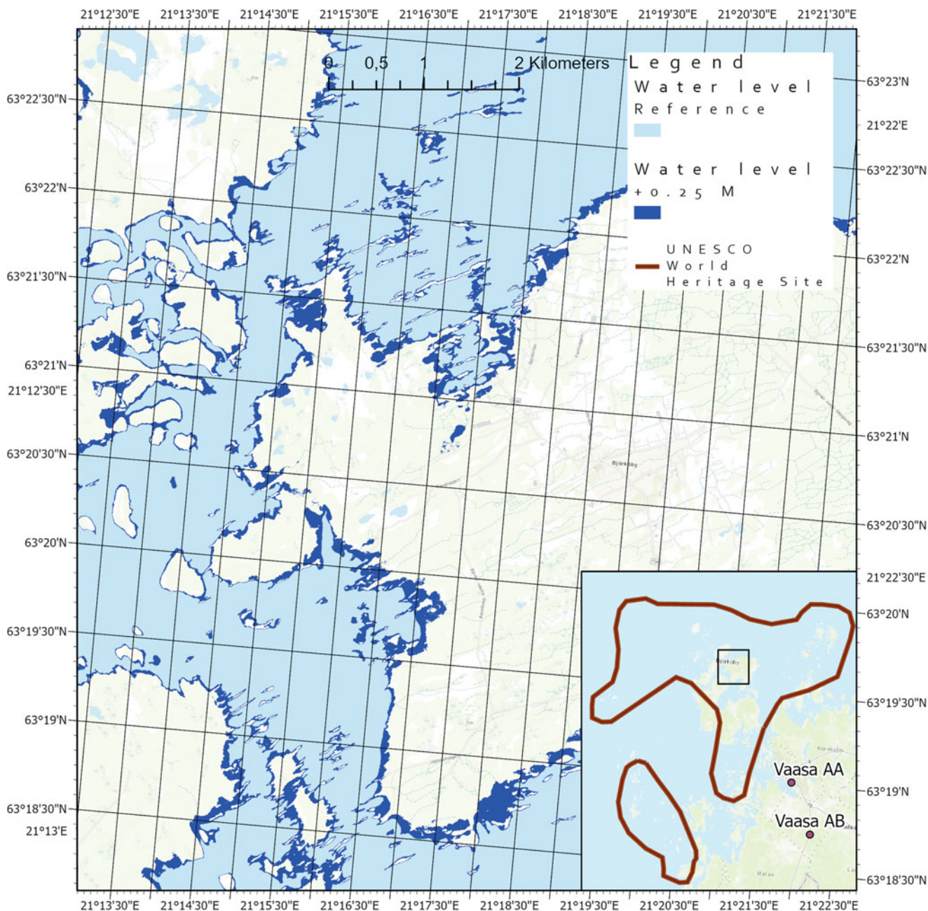
Fig. 2 The future scenario of Table 2 plotted for Kvarken's Björkö. The light blue shows the present coast line, and the dark blue the 95% probability scenario (sea level rise of 25 cm)
