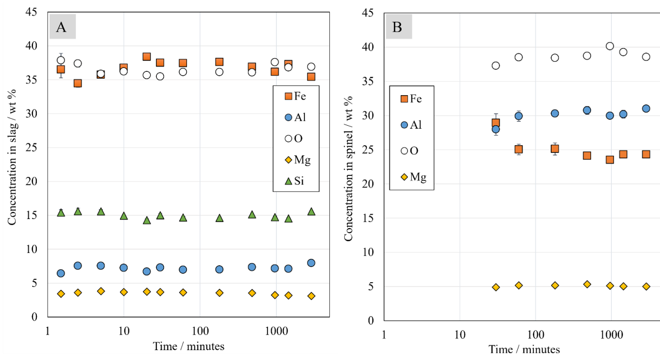
Figure 4. Concentrations of major elements in the slag (A) and spinel (B) phase as a function of time.
