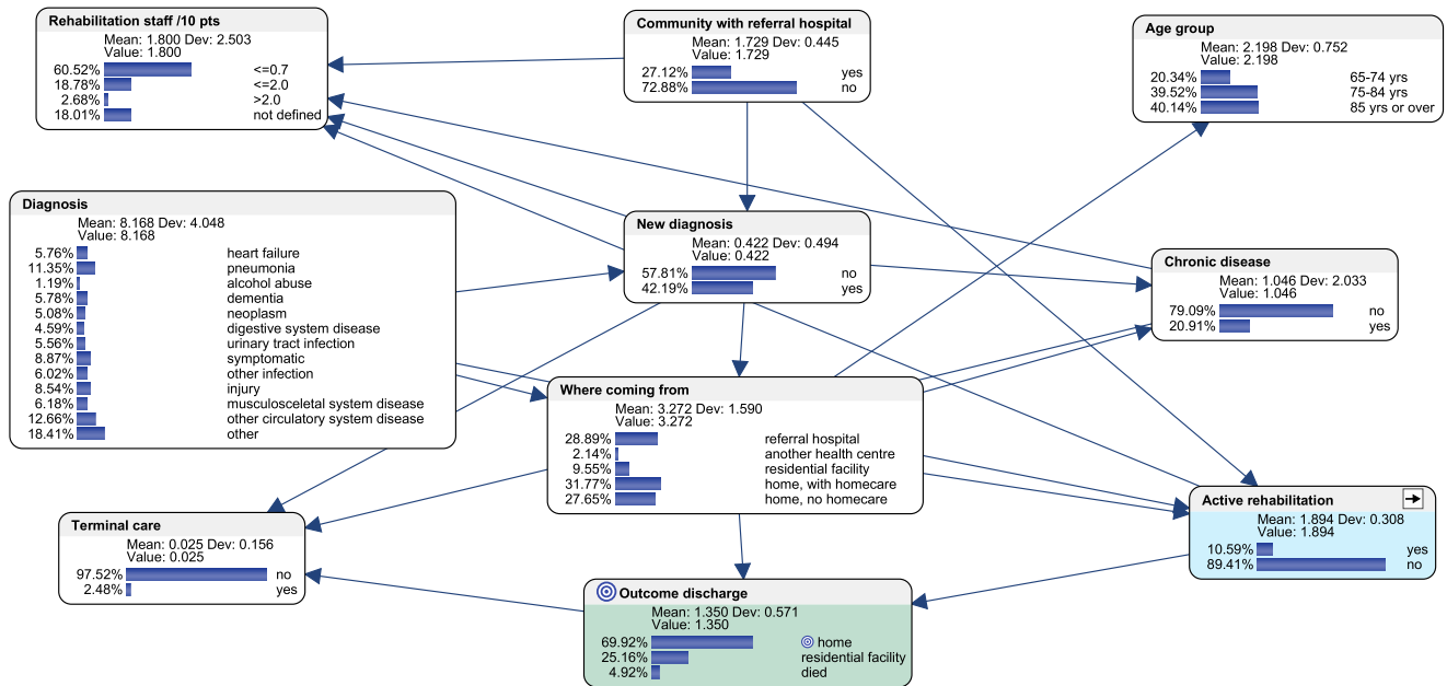
Fig. 1. Bayesian Network Model. Variables associated with the outcome variable Outcome discharge or intervention variable Active rehabilitation . Variables are presented with a conditional probability table (CPT).
