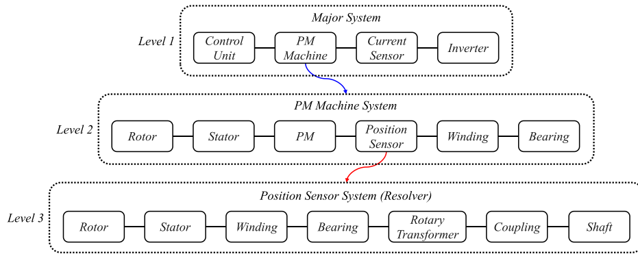
FIGURE 1. Reliability block diagram of the PMM drive system.
