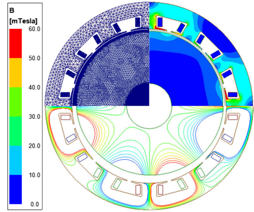
FIGURE 10. Schematic of the mesh grid, magnetic flux density, and magnetic flux lines on the studied 1-X VR resolver with CTNOW configuration.
