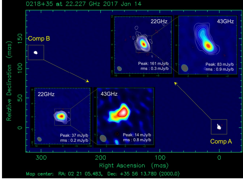
Figure 1: KaVA radio view of the source. The radio interferometry zoom to the two image components A and B is shown in inset panels.
