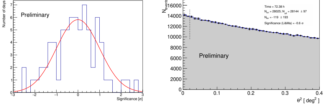
Figure 2: Left panel: distribution of significances of individual nights of MAGIC observations, for reference the red line shows a Gaussian distribution with a mean of 0 and standard deviation of 1. Right panel: Distribution of the squared angular distance between the nominal and reconstructed position of QSO B0218+357 (points) and corresponding background estimation (shaded region).
